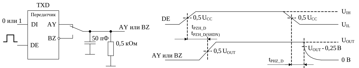
а) t_{PZH\_D} , t_{PHZ\_D} и t_{PZH\_D(SHDN)}
