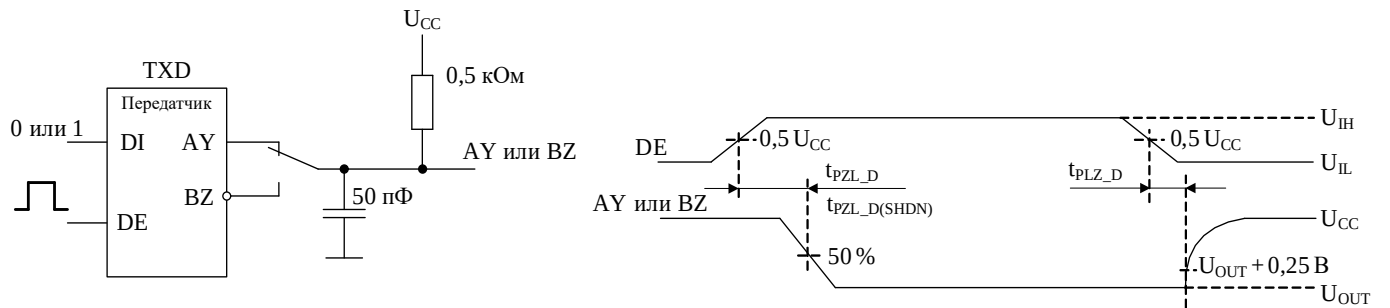
б) t_{PLZ\_D} , t_{PLZ\_D} и t_{PLZ\_D(SHDN)}
