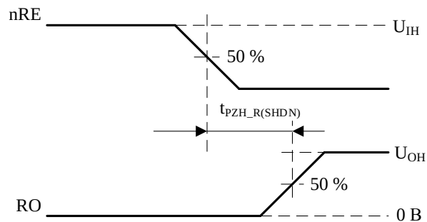
а) t_{PZH\_R(SHDN)}
